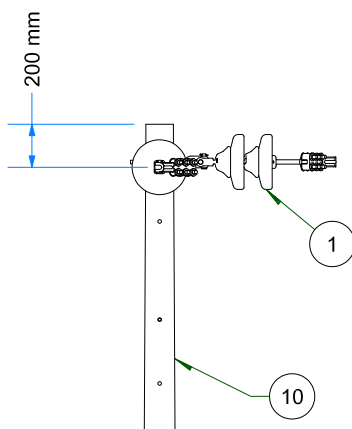
VISTA FRONTAL SCALE 1 / 35
